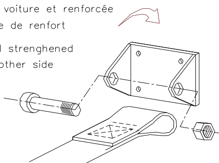
Dessin / Drawing 253-63
