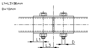
Drawing 253-42
