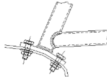
Drawing 253-57
